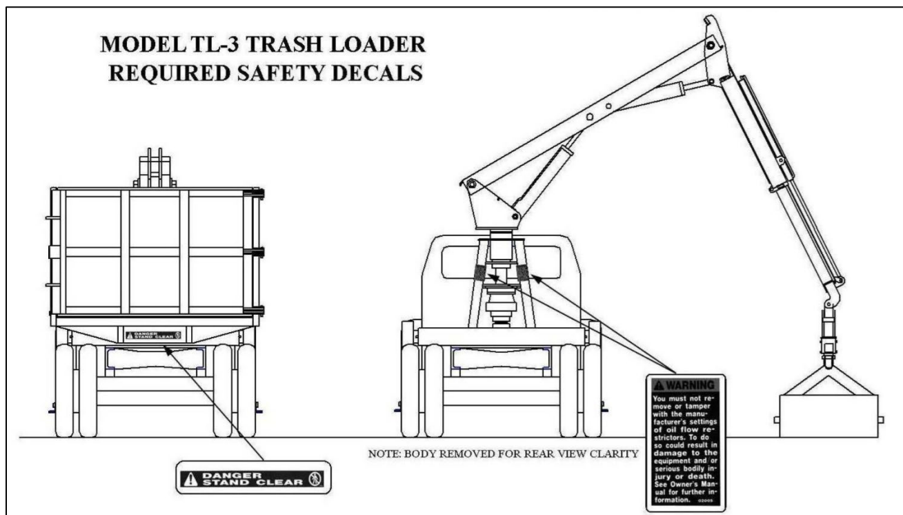
Safety Decal Locations
